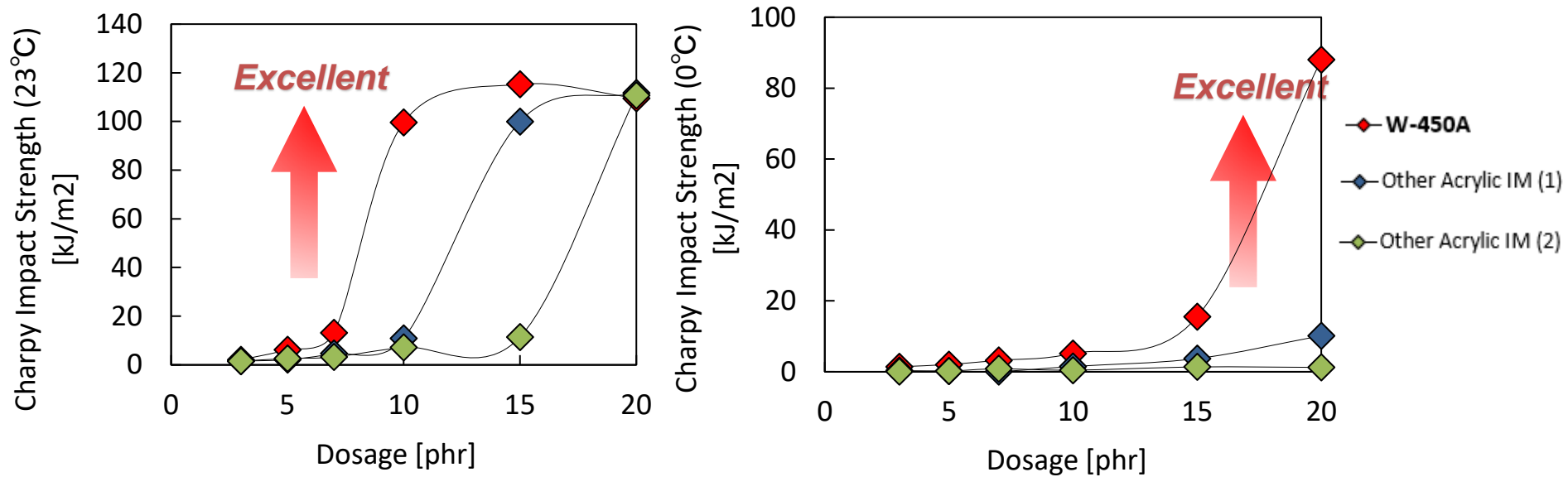
Fig. Charpy impact strength of PVC.
