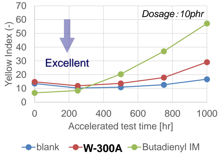
Fig. Weatherability of PVC.
