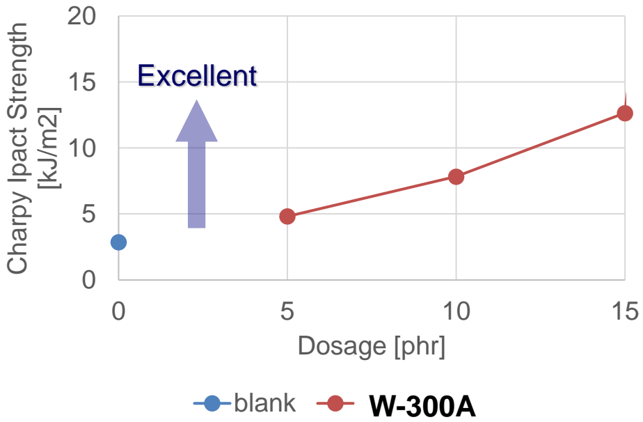
Fig. Charpy impact strength of PVC.
