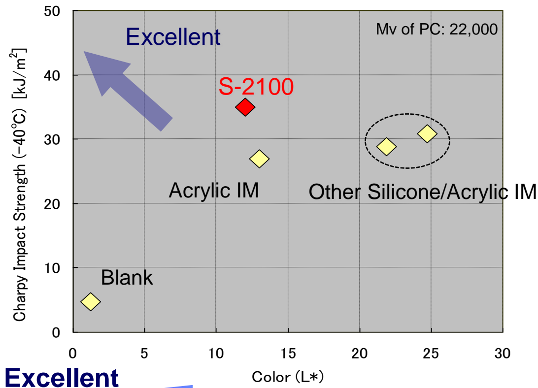
Fig. Colorability - Charpy impact strength balance of S-2100.
