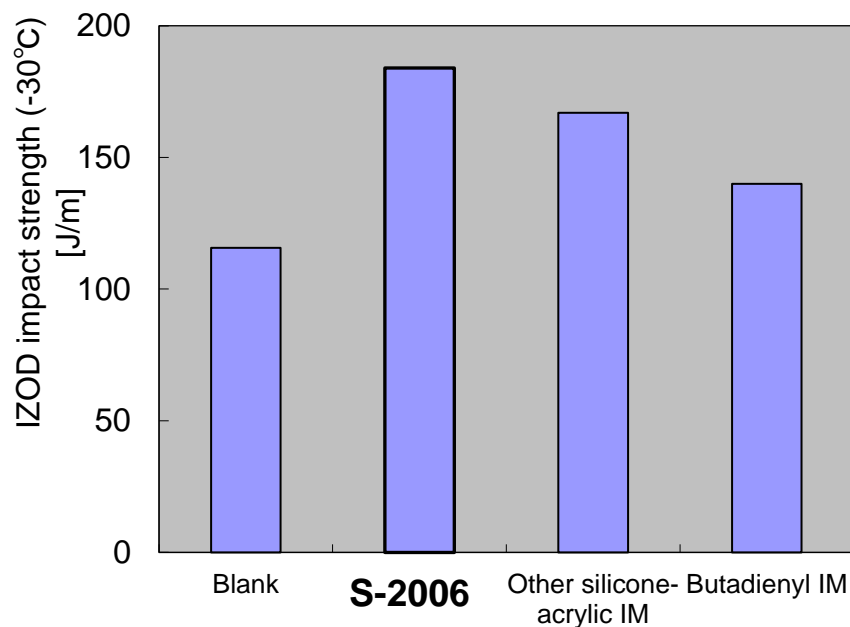
IZOD Impact Strength (at -30°C)
