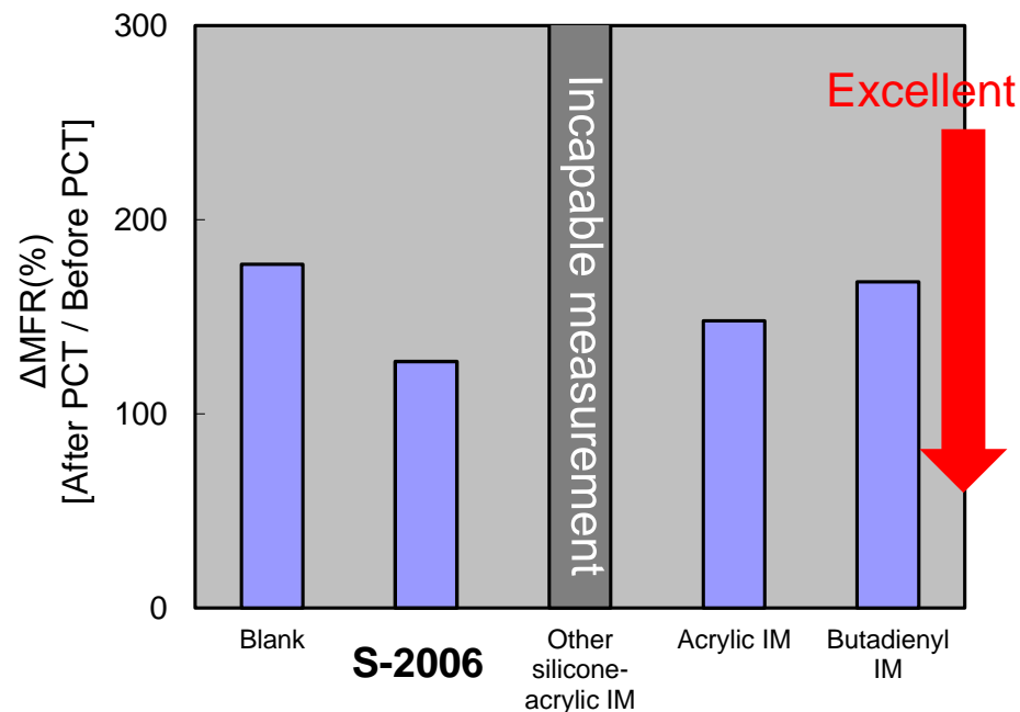
Melt Flow Rate After Hydrolysis
